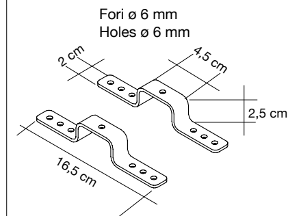
Dettaglio attaches Brackets detail
